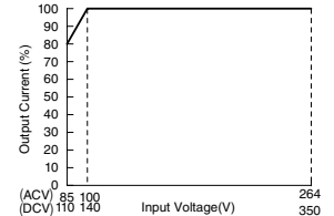
Overcurrent Protection Characteristics PS9Z-6RM*
