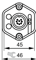
End View
